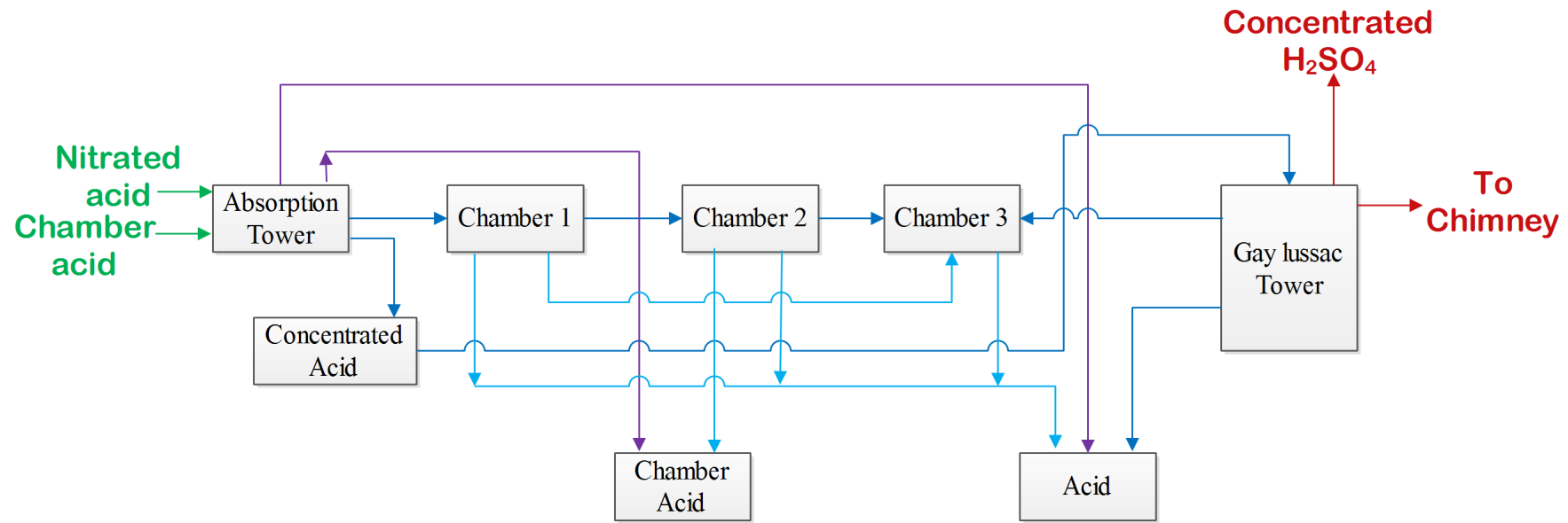
Figure: Manufacturing of Sulfuric acid by Chamber process
